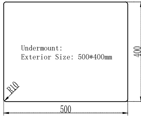
Undermount Installation
