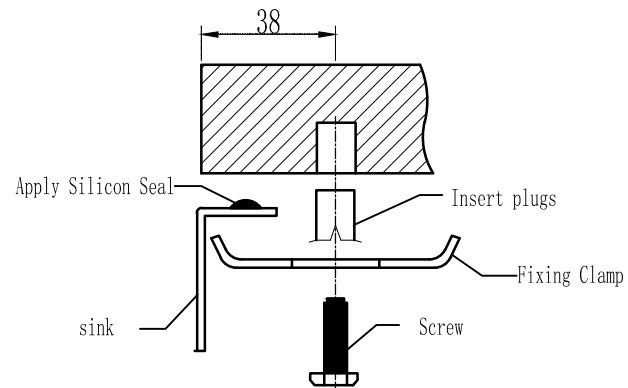
UNDERMOUNT INSTALLATION
