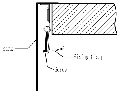
TOPMOUNT INSTALLATION
