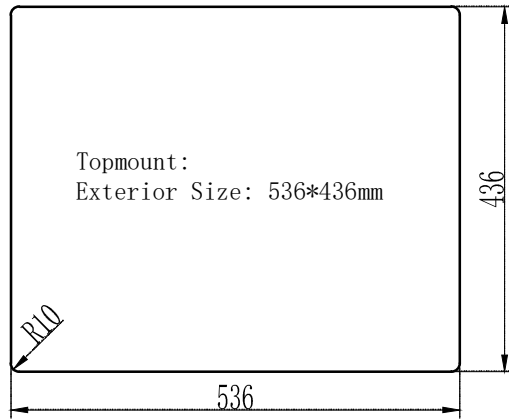
Topmount Installation
